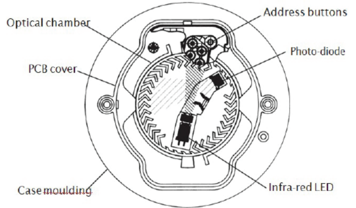
Top Section - DS-0D02 Optical smoke detector
